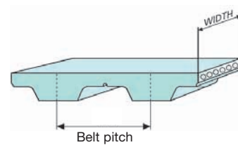
Reference dimensions
