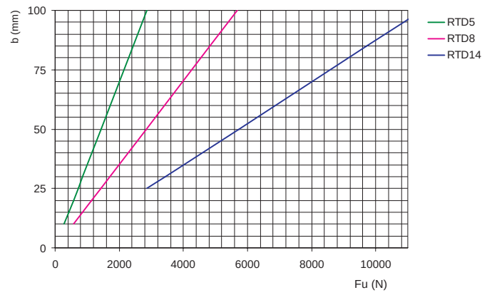
RTD profile
